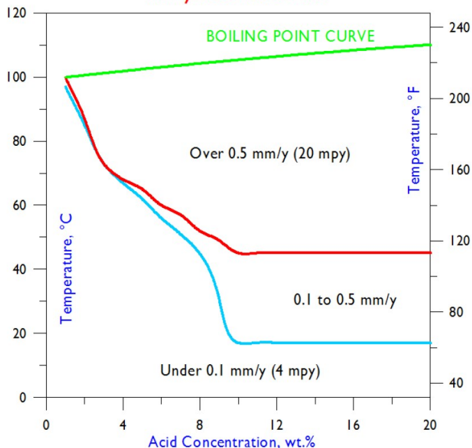
Iso-Corrosion Diagram for Alloy 625 in Hydrochloric Acid
