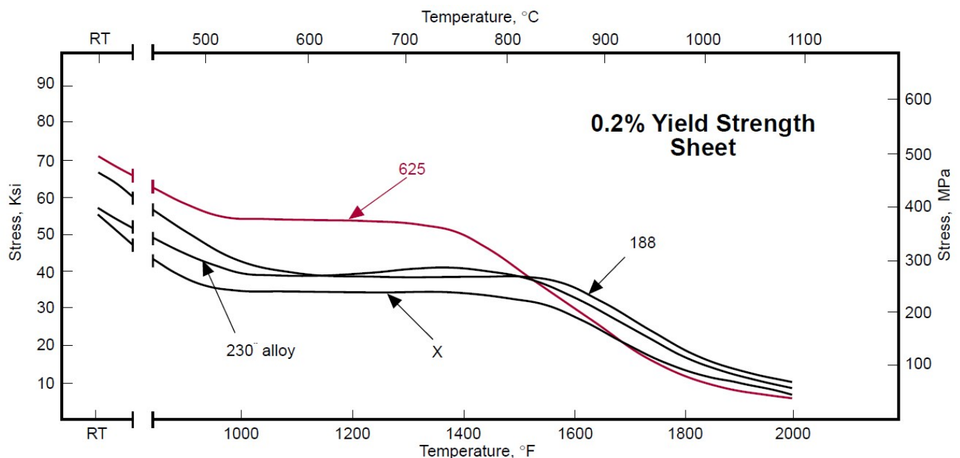
Comparative Elevated Temperature Yield Strengths, Sheet
